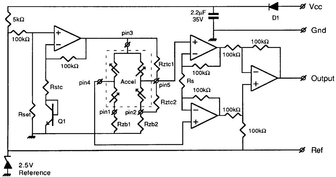
Figure 1. Typical Temperature Compensation and Amplification Circuit (component values specified for each sensor)
